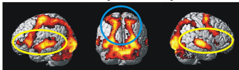
Figure 2. Whole-brain voxel-wise random effects statistical parameter maps of each condition contrasted with the fixation baseline thresholded at p < .0001 with an 81-voxel extent threshold (resulting in a cluster-level threshold of p < .05 after correction for multiple comparisons). Similar areas of activation are present in both conditions but with additional language-related activity in temporal and inferior frontal areas (yellow ovals).
